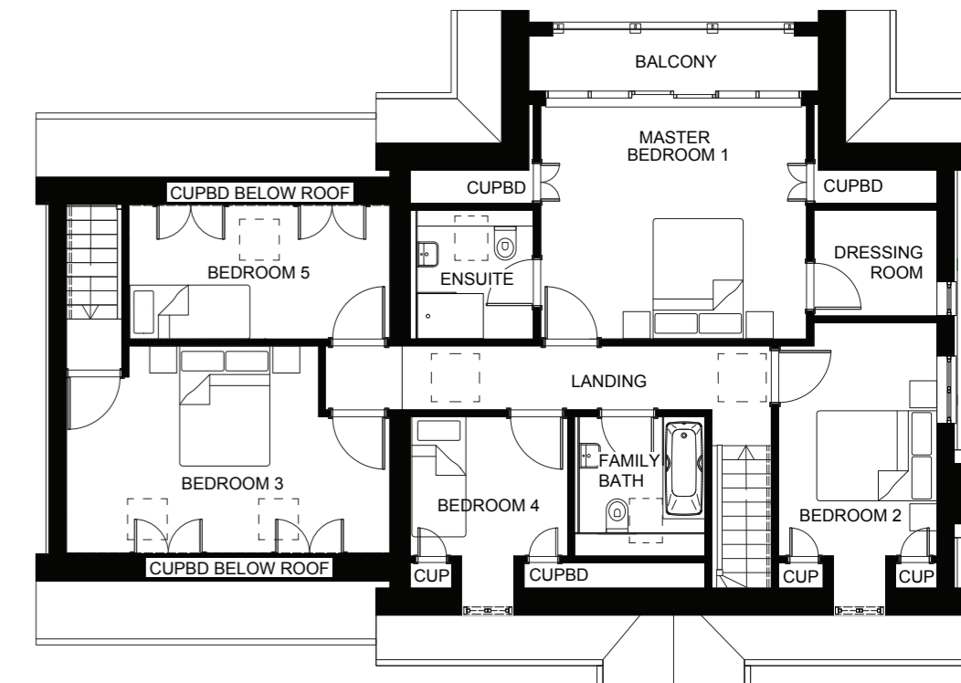
First Floor
